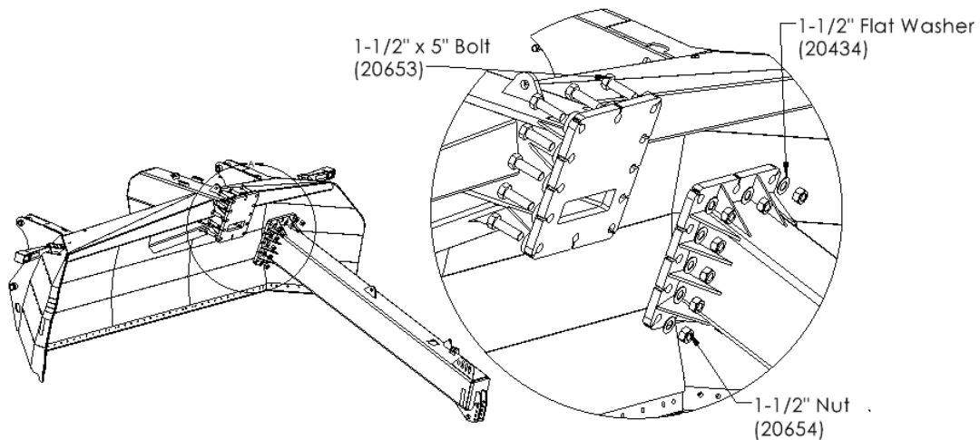
Figure 1 - Blade to hitch Attachment
