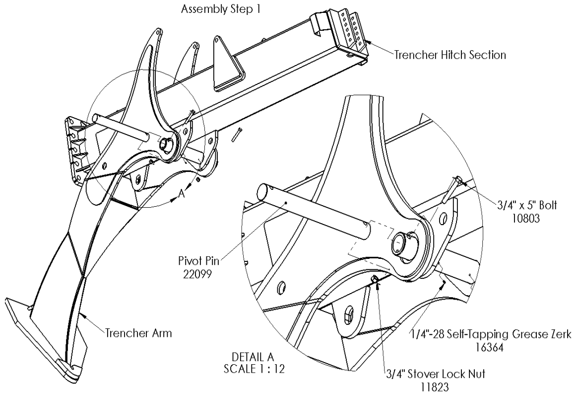
Figure 33 - Trencher install
