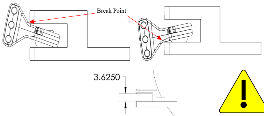
Figure 2.1 – Articulation clearance
